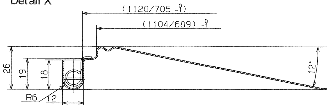
Detail X
