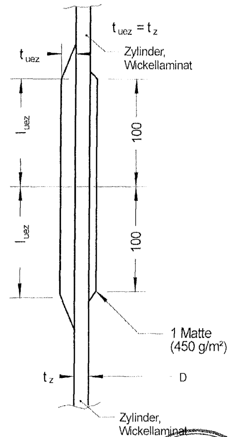
Detail C
