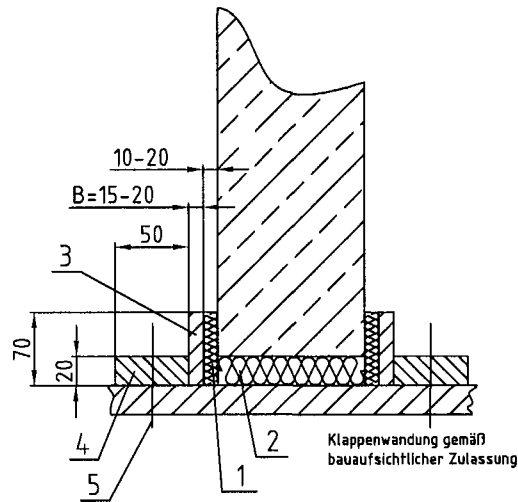
Detail A
