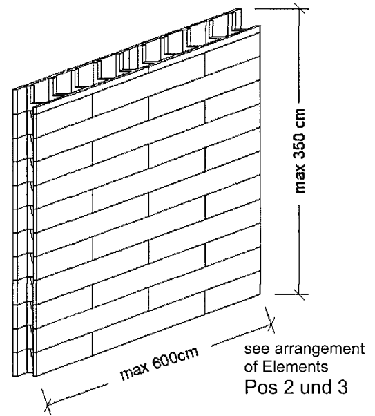
normal element
