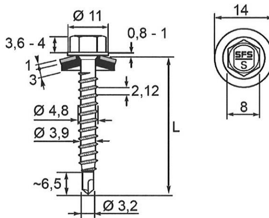
Schraube SW2-S-A14-4,8x35
