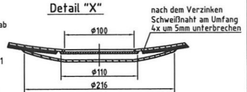
Detail "X"
