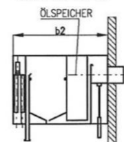
Detail NS 15-24
