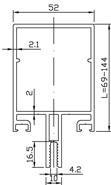
Riegel 52T83 L=69mm 52T84 L=84mm 52T85 L=104mm 52T87 L=124mm 52T86 L=144mm
