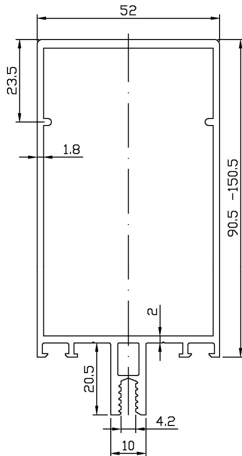
Riegel 52T54 L=60 mm 52T62 L=90,5mm 52T60 L=110,5mm 52T61 L=130,5mm 52T63 L=150,5mm
