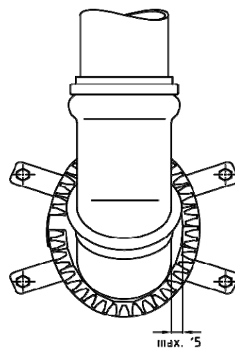
View A
