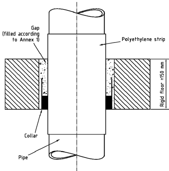
Collar full mortared into the floor
