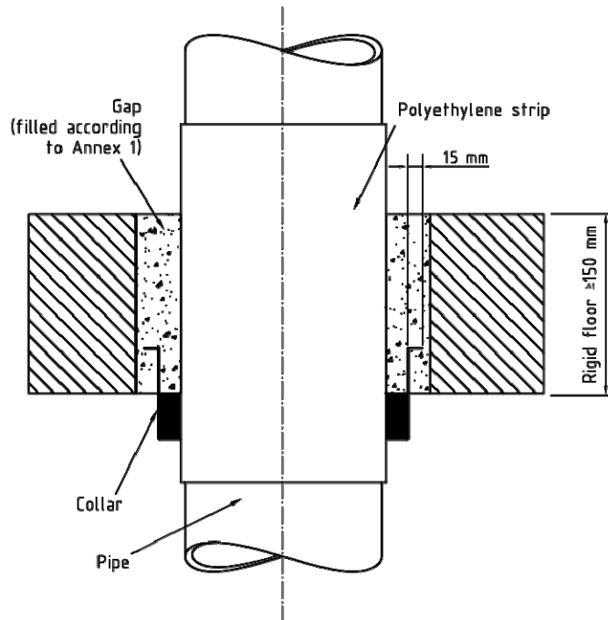
Fixing strap mortared into the floor
