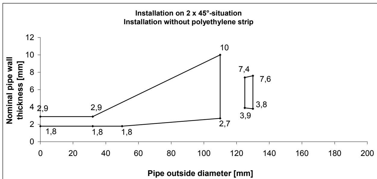
Figure 12 – EI 90-U/C (floor installation)
