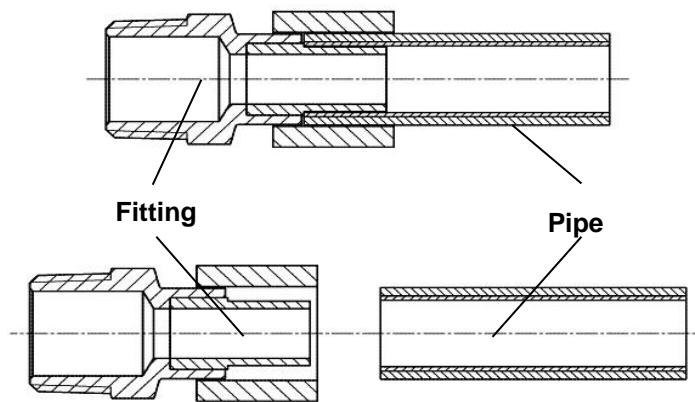
Figure 1: Piping System
