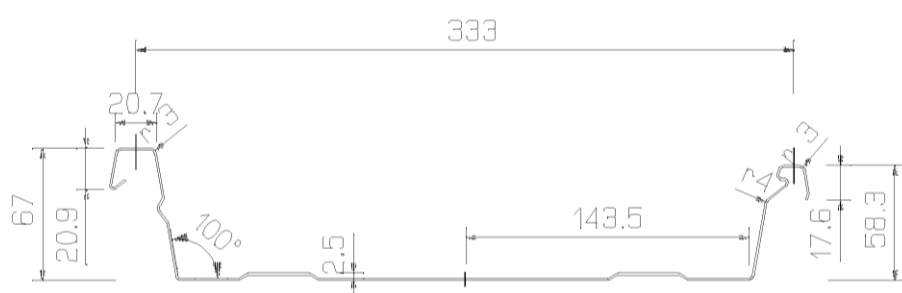
RIB-ROOF Speed 500 Baubreite = 333 mm
