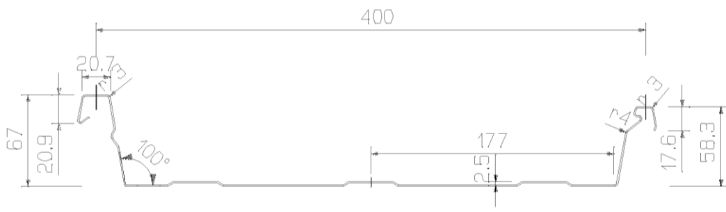
RIB-ROOF Speed 500 Baubreite = 400 mm
