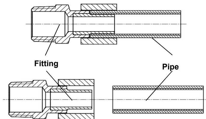
Figure 1: Piping System
