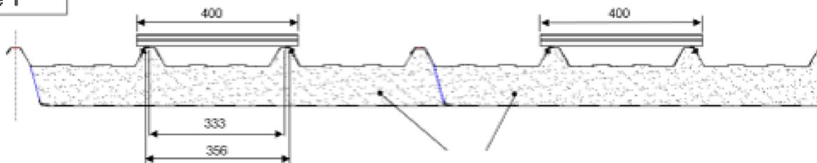
Sandwich-Dachelement REX SDW ROOF 3
